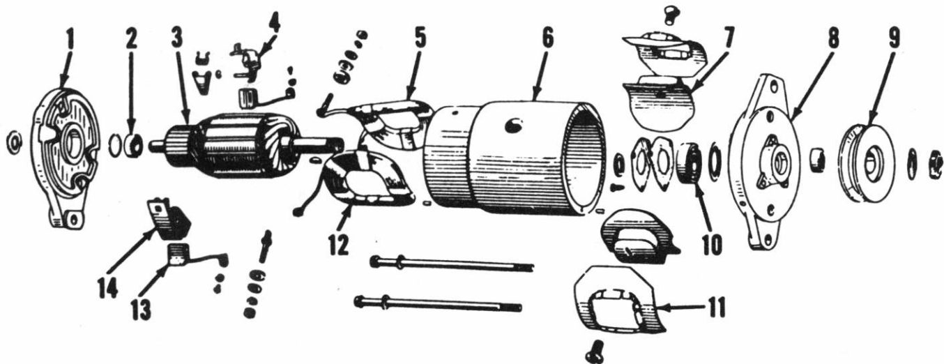
Fig. W38—Exploded view of typical Delco-Remy starter-generator.
